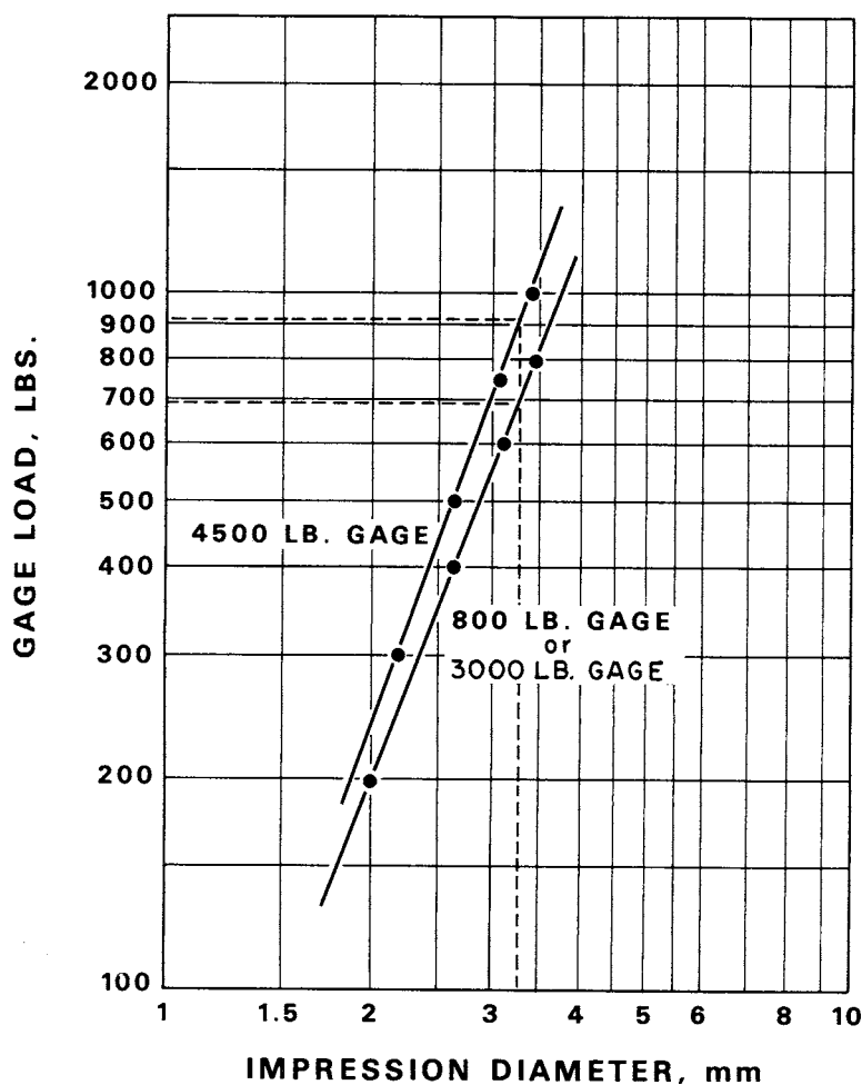
FIG. 5 Typical Curves of Gage Load Readings versus Impression Diameter, Using 800, 3000 and 4500-lb Gages and BHN 37 to 39 Standard Test Coupons
