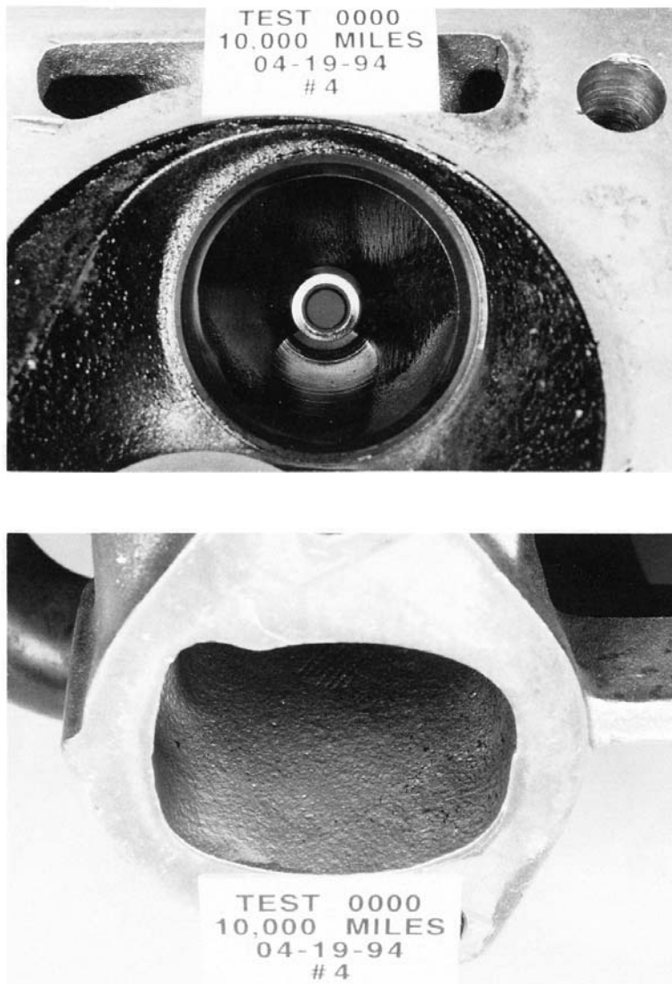
FIG. 13 Typical Photographs of Intake Ports and Runners
