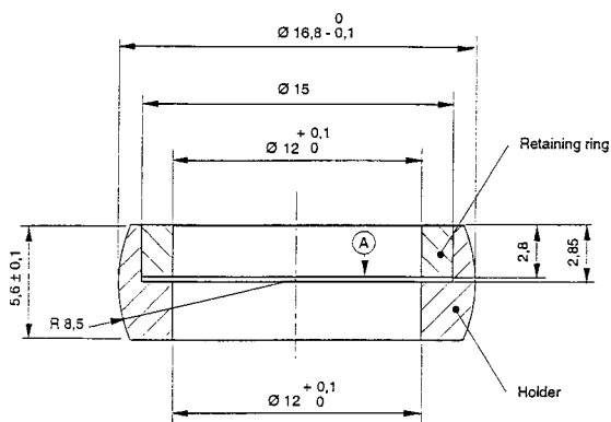
FIG. 7 Filter Unit
