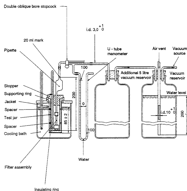
FIG. 1 Arrangement of Manual CFPP Apparatus
