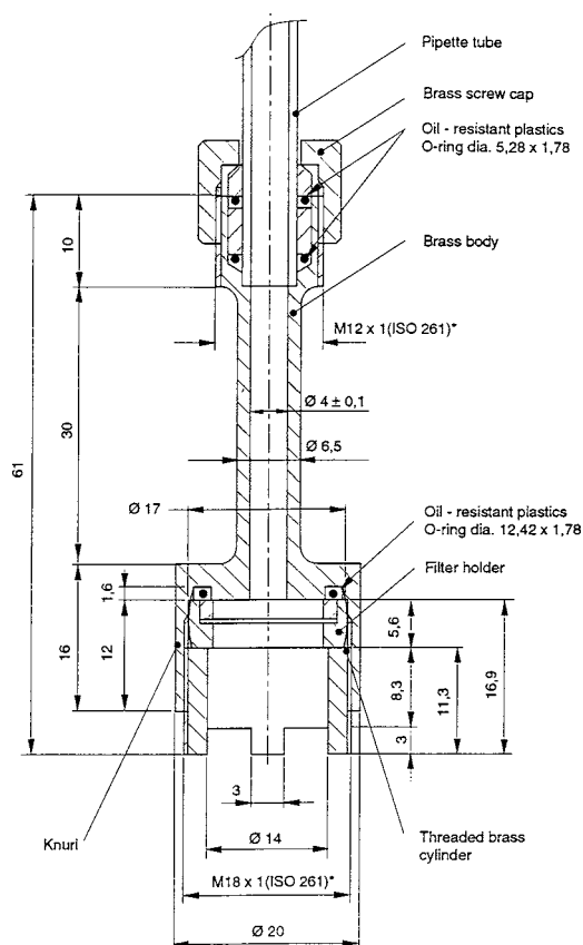
FIG. 7 Filter Unit
