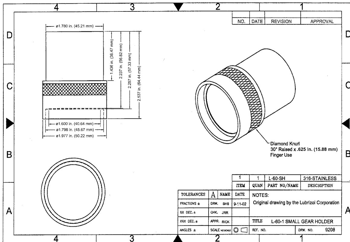
FIG. A9.1 Small Gear Holder
